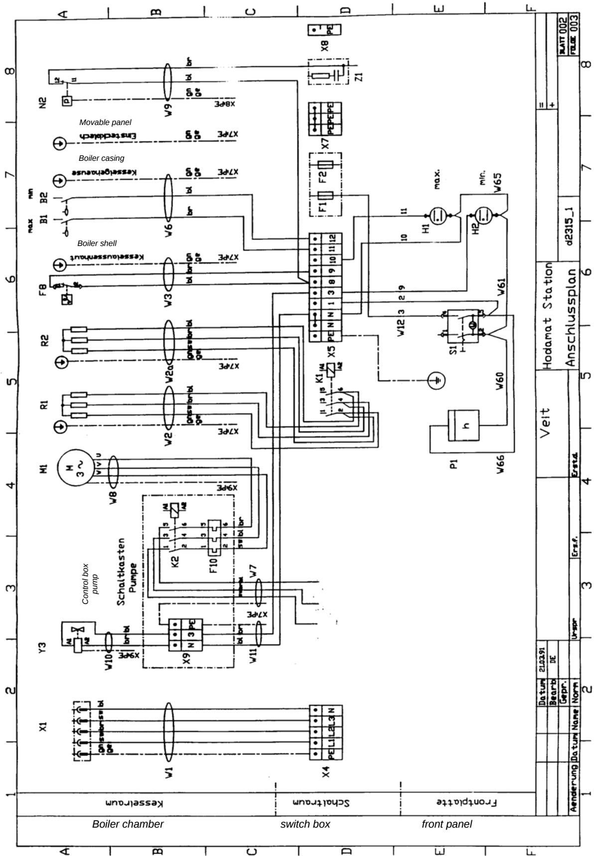
Connection Plan
